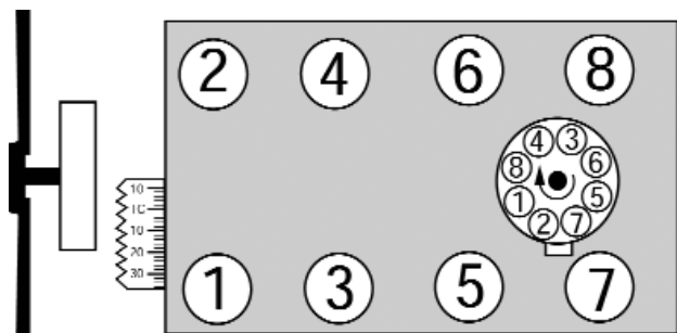
Figure 1- Chevrolet 396-454 c.i.d. V8
