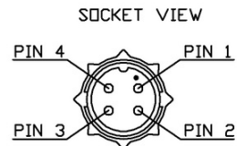
HARNESS CONNECTOR #37-1531
