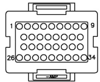
LCU CONNECTOR 34 PIN VIEW FROM WIRE SIDE
